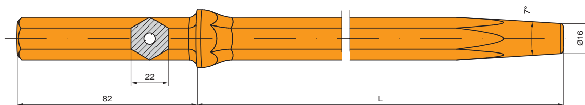
Tapered rod, shank Hex 22 x 82 mm
