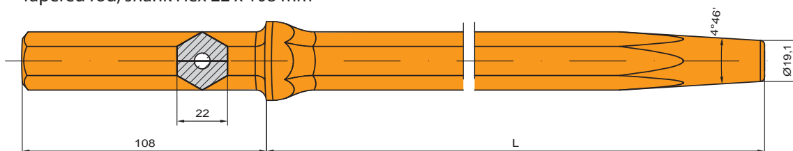
Tapered rod, shank Hex 22 x 108 mm
