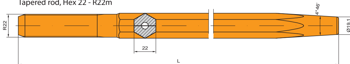
Tapered rod, Hex 22 - R22m
