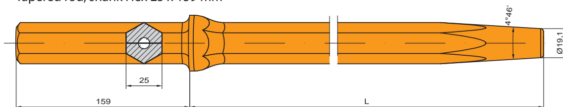
Tapered rod, shank Hex 25 x 159 mm
