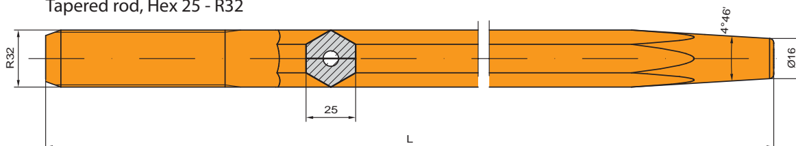
Tapered rod, Hex 25 - R32
